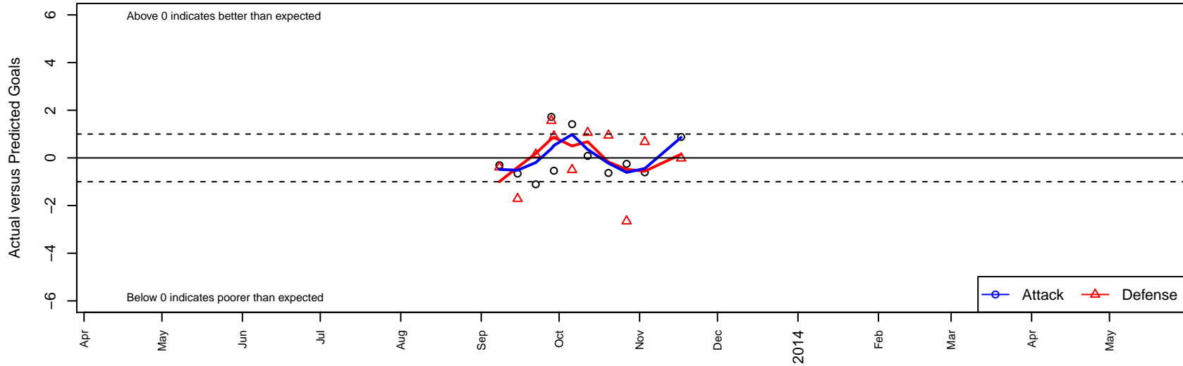
OC Premier Black B96 Dots are actual minus expected GF (blue circles) and GA (red triangles). Blue line is smoothed change in attack strength. Red is smoothed change in defense strength.
